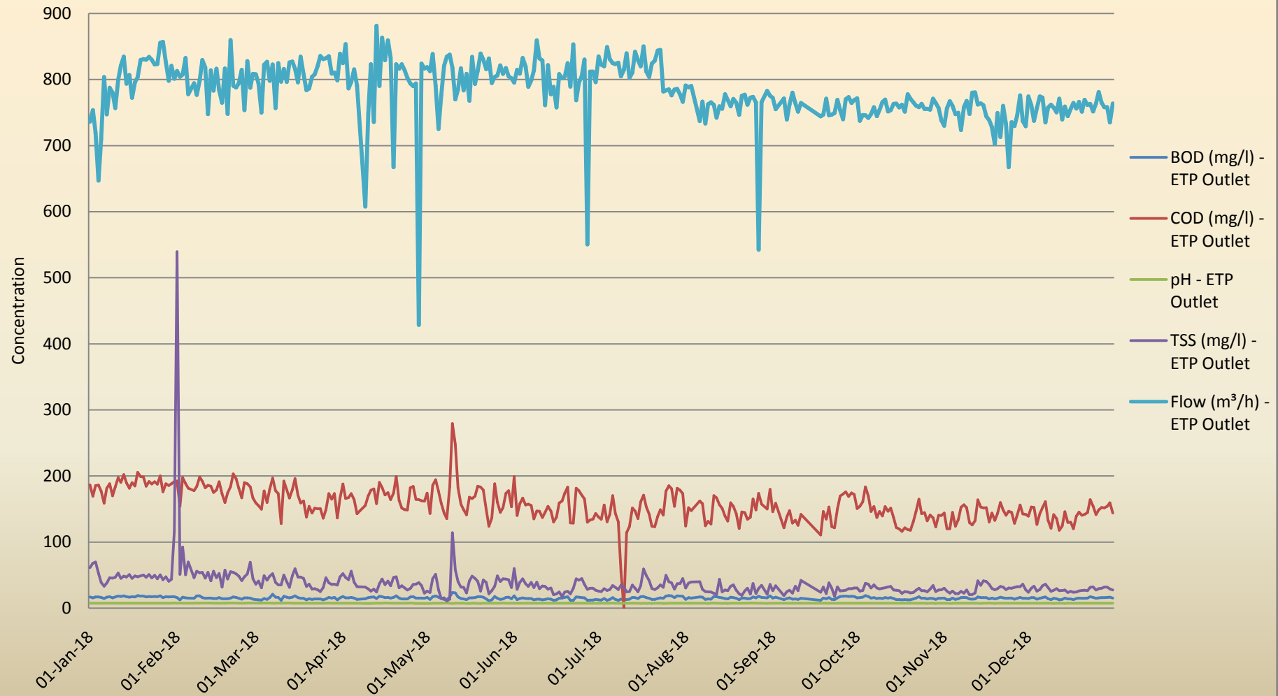
Annual Effluent Trend in M/s. Grasim Industries Ltd., Dist. Ujjain (M.P.)
